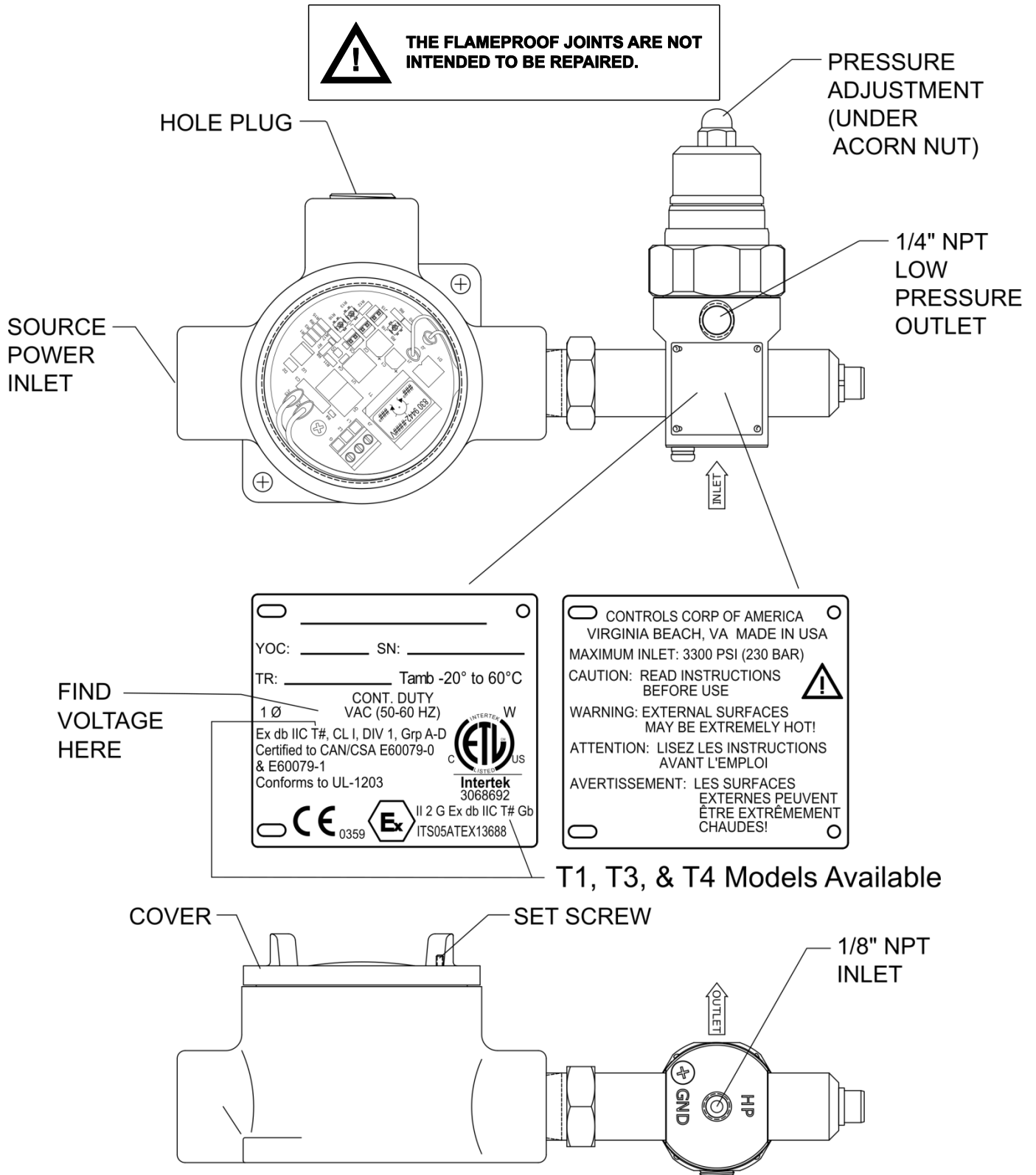
Figure 1 – Vaporizing Regulator Assembly
